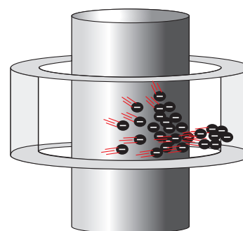
Townsend Avalanche of Gaseous Ions
