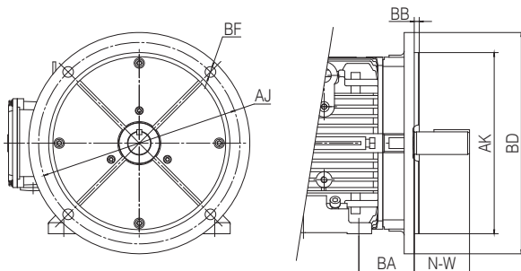
Figure 4 - D-Flange
