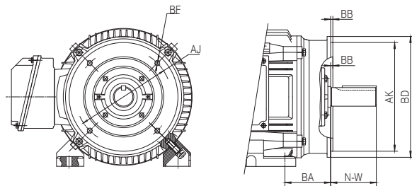
Figure 2 - C-Flange
