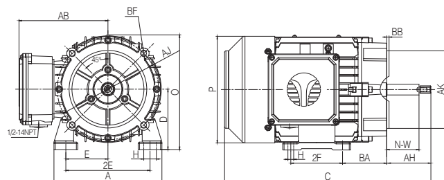
Figure 1 - Foot Mount, 56J
