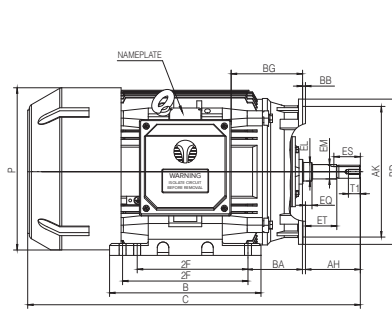
Figure 2 - Cast Iron JM/JP Model
