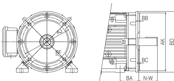
Figure 3 - C-Flange
