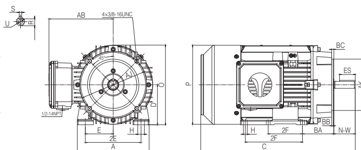
Figure 2 - Foot Mount, 56HC
