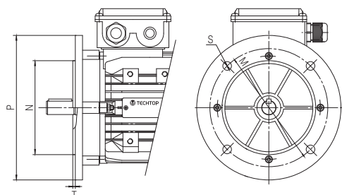
Figure 4 - D-Flange B5/B5R
