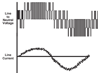
Figure 1 PWM Waveform
